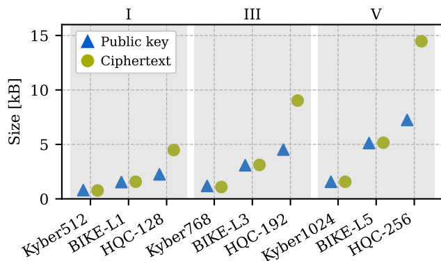
Fig. 6: Public key and ciphertext sizes of the benchmarked post-quantum KEMs grouped by NIST level.
